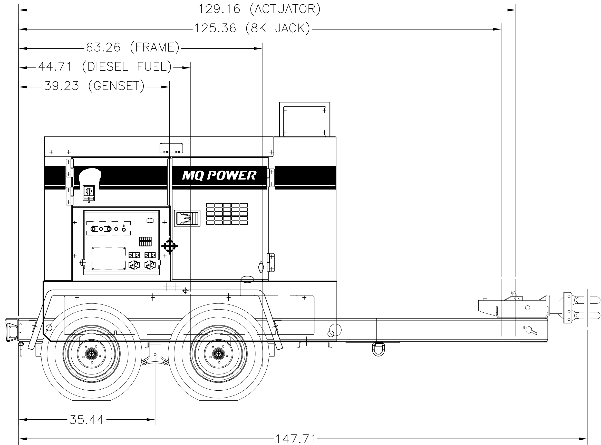
DCA40SSKU4F MOUNTED ON TRLR45H TRAILER (DWG NO. 201978)
